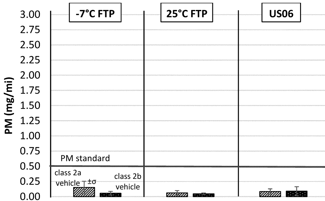
Figure 14: PM Measurements Comparing PM From a Class 2a Vehicle to a Class 2b Vehicle, Both With MY 2022 GPFs, in -7^{\circ}\text{C} FTP, 25^{\circ}\text{C} FTP, and US06 Test Cycles
